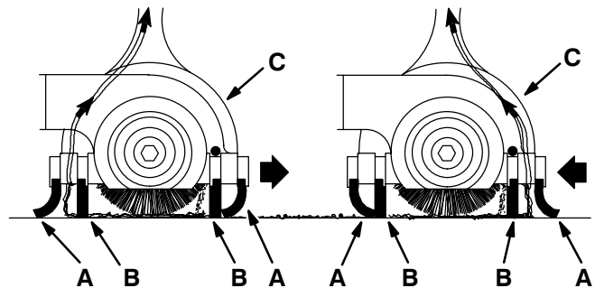
SQUEEGEE ADJUSTMENT
