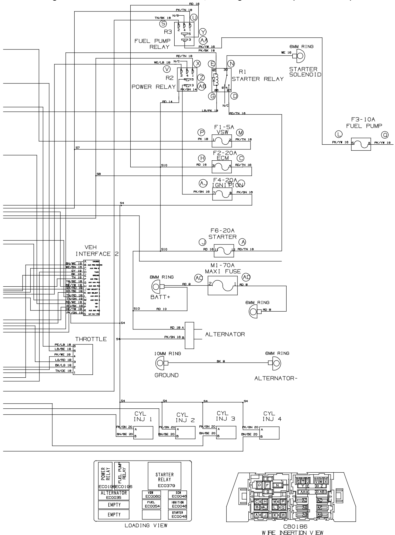
Fig. 82 - Mitsubishi Electrical Schematic, Gas Engine Harness (004000- )
