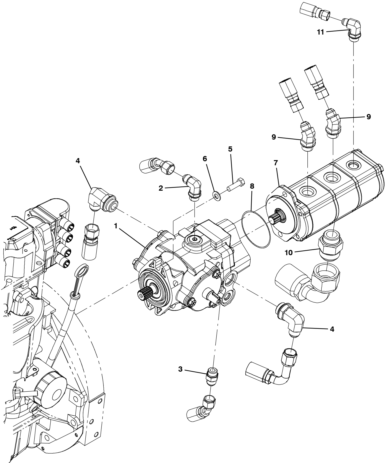
Fig. 71 - Hydraulic Pumps Group
