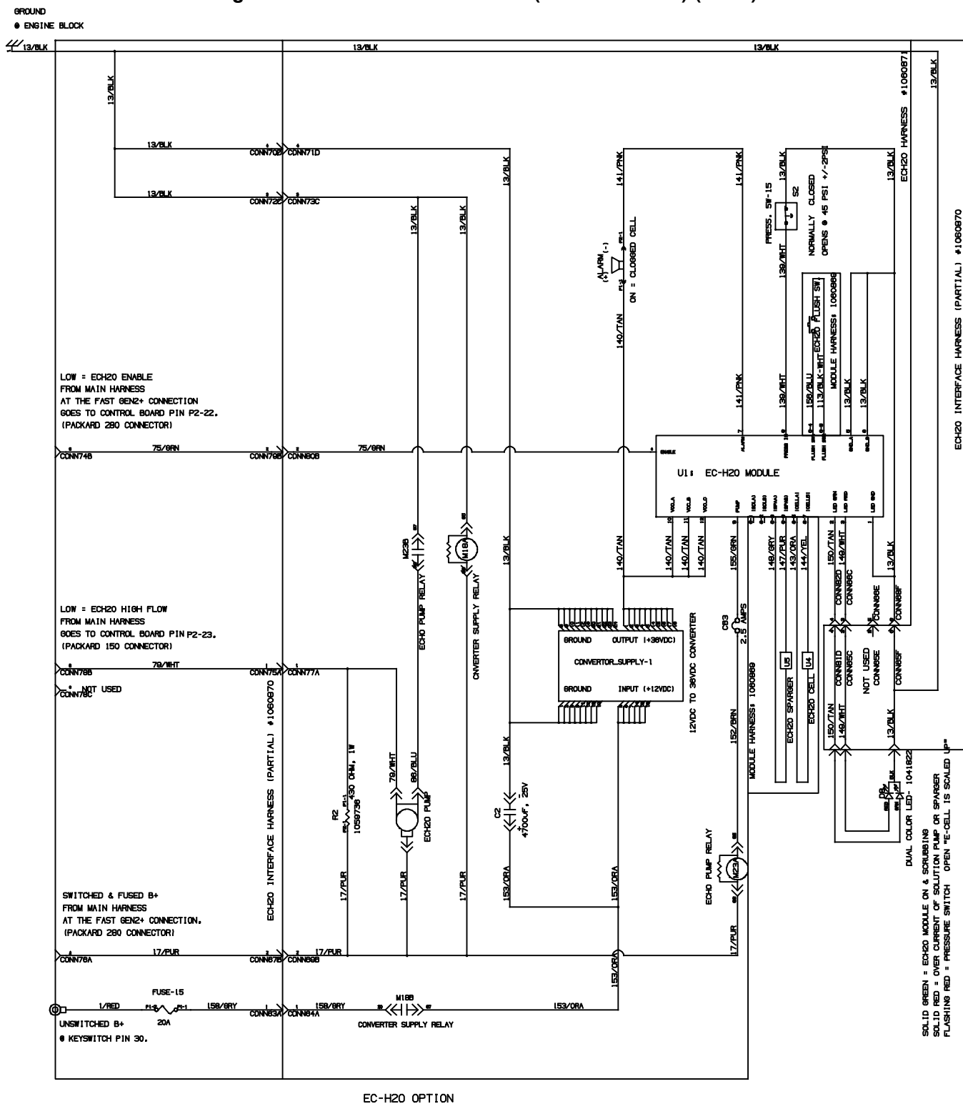
Fig. 76 - GM Electrical Schematic (001545-003999) (7 of 7)
