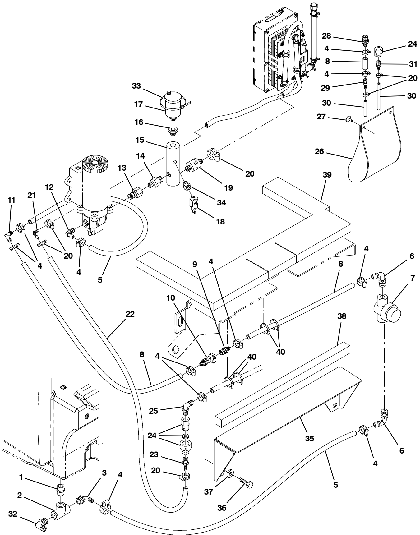
Fig. 14 - ec-H2O Solution Pump Supply Group
