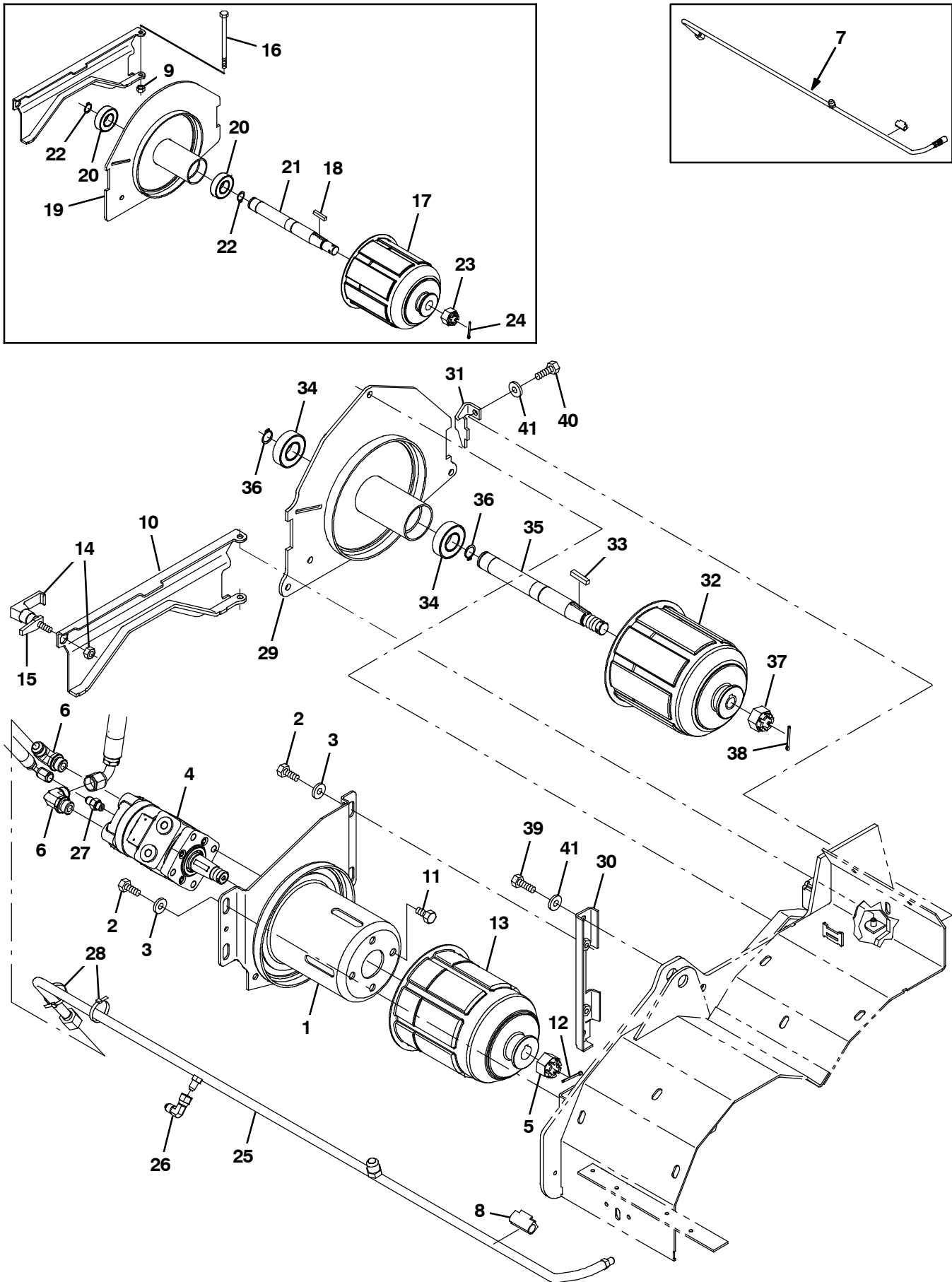
Fig. 48 - Brush Drive Group, Right Side
