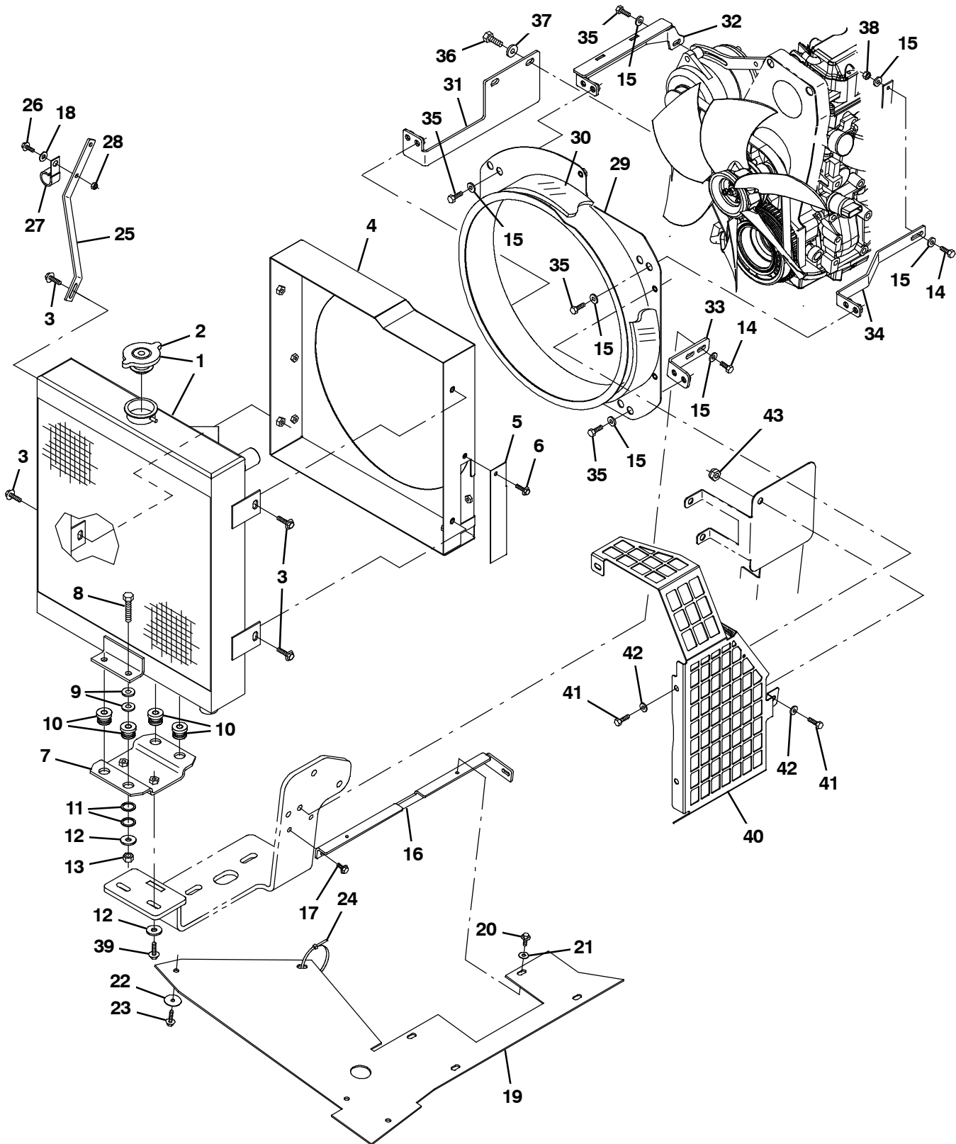
Fig. 22 - GM Engine Radiator and Mount Group (001250-003999)
