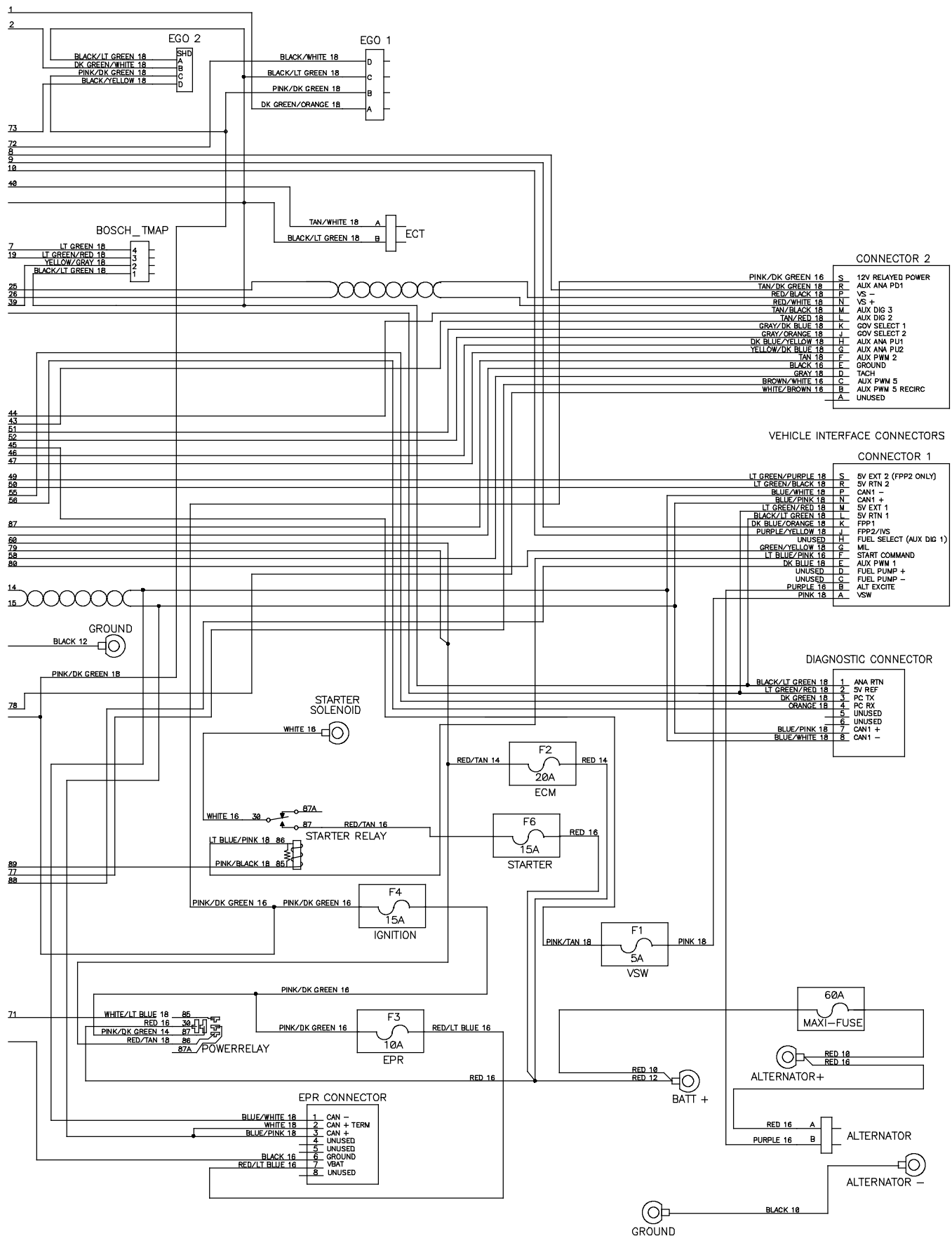
Fig. 79 - GM Electrical Schematic, LPG Engine Harness (000000-001320)
