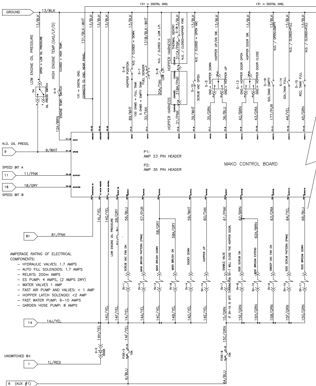
Fig. 75 - GM Electrical Schematic (000000-001544) (3 of 7)
