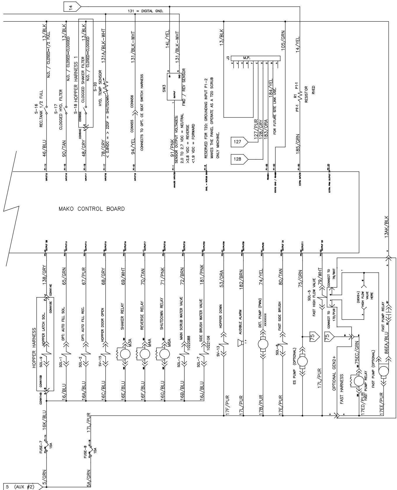
Fig. 75 - GM Electrical Schematic (000000-001544) (4 of 7)
