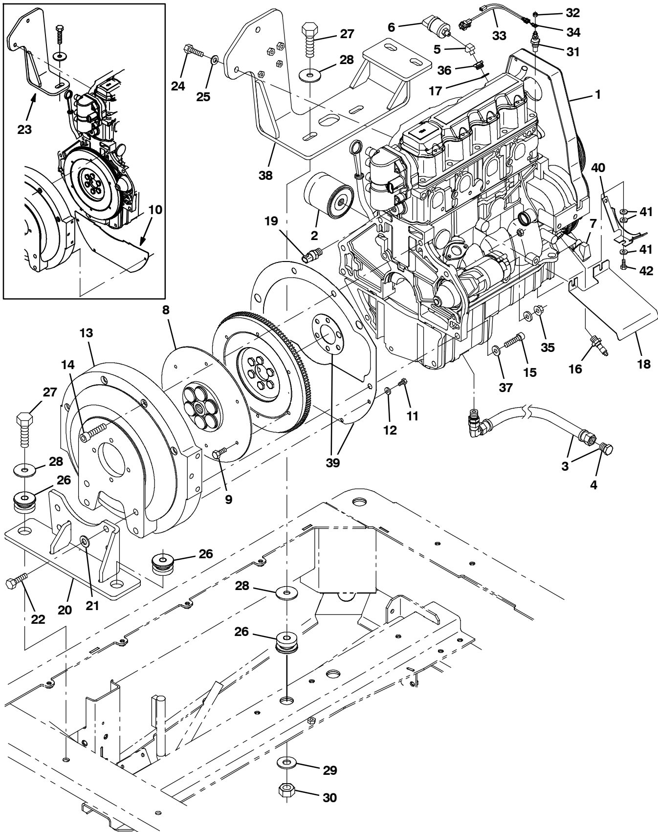
Fig. 11 - GM Engine and Mount Group (000000-003999)
