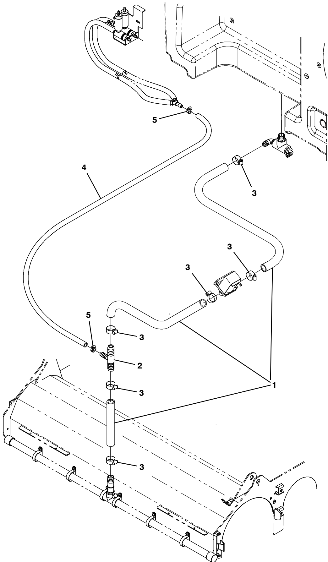
Fig. 10 - FaST Solution Supply Group
