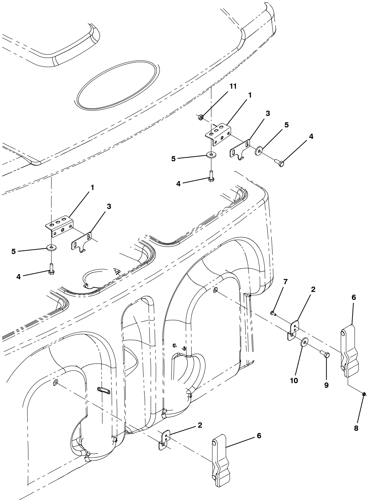
Fig. 31 - Transport Group
