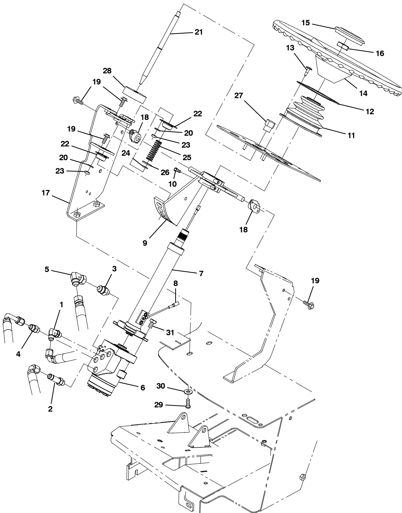
Fig. 8 - Steering Group
