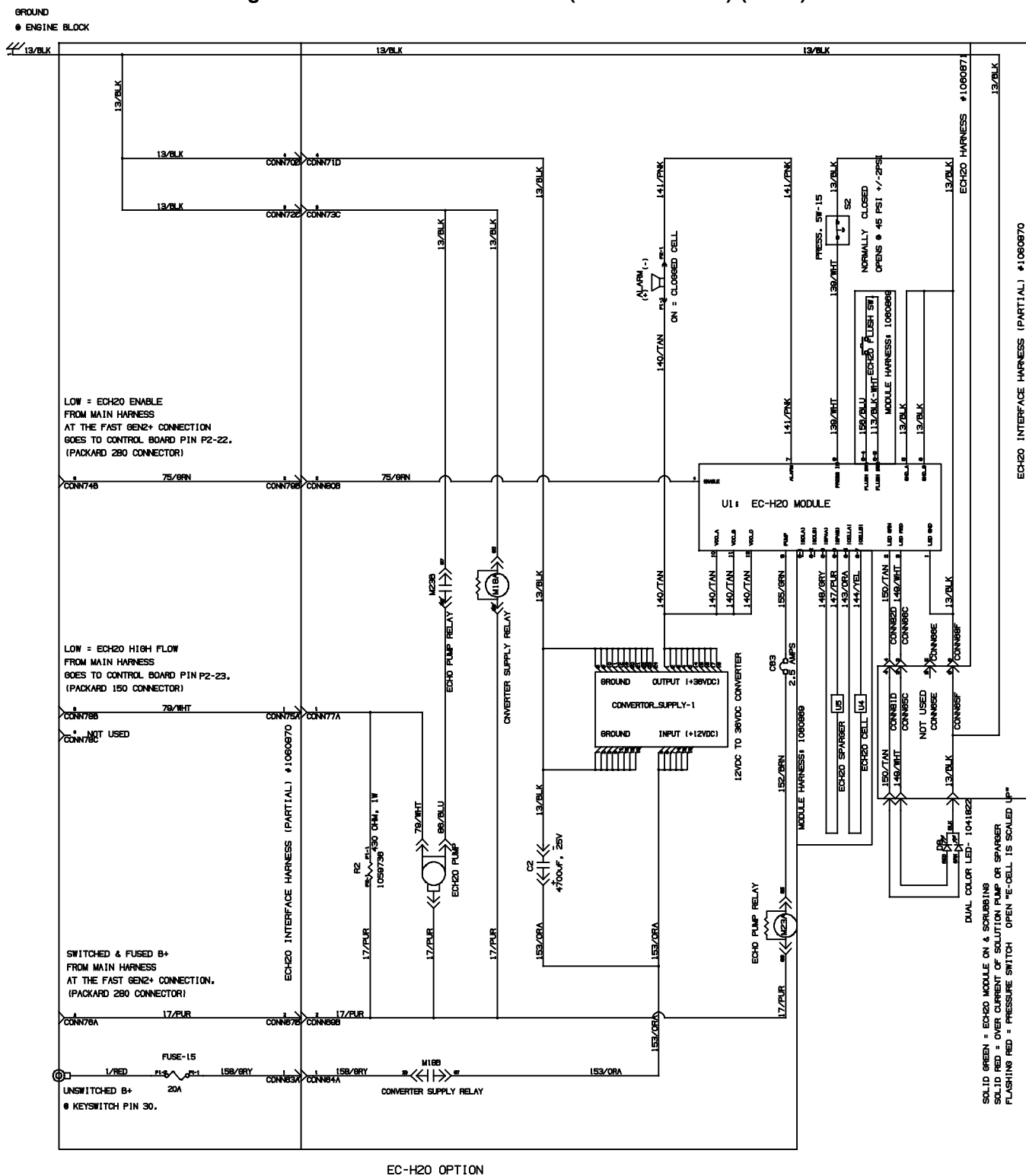
Fig. 75 - GM Electrical Schematic (000000-001544) (7 of 7)
