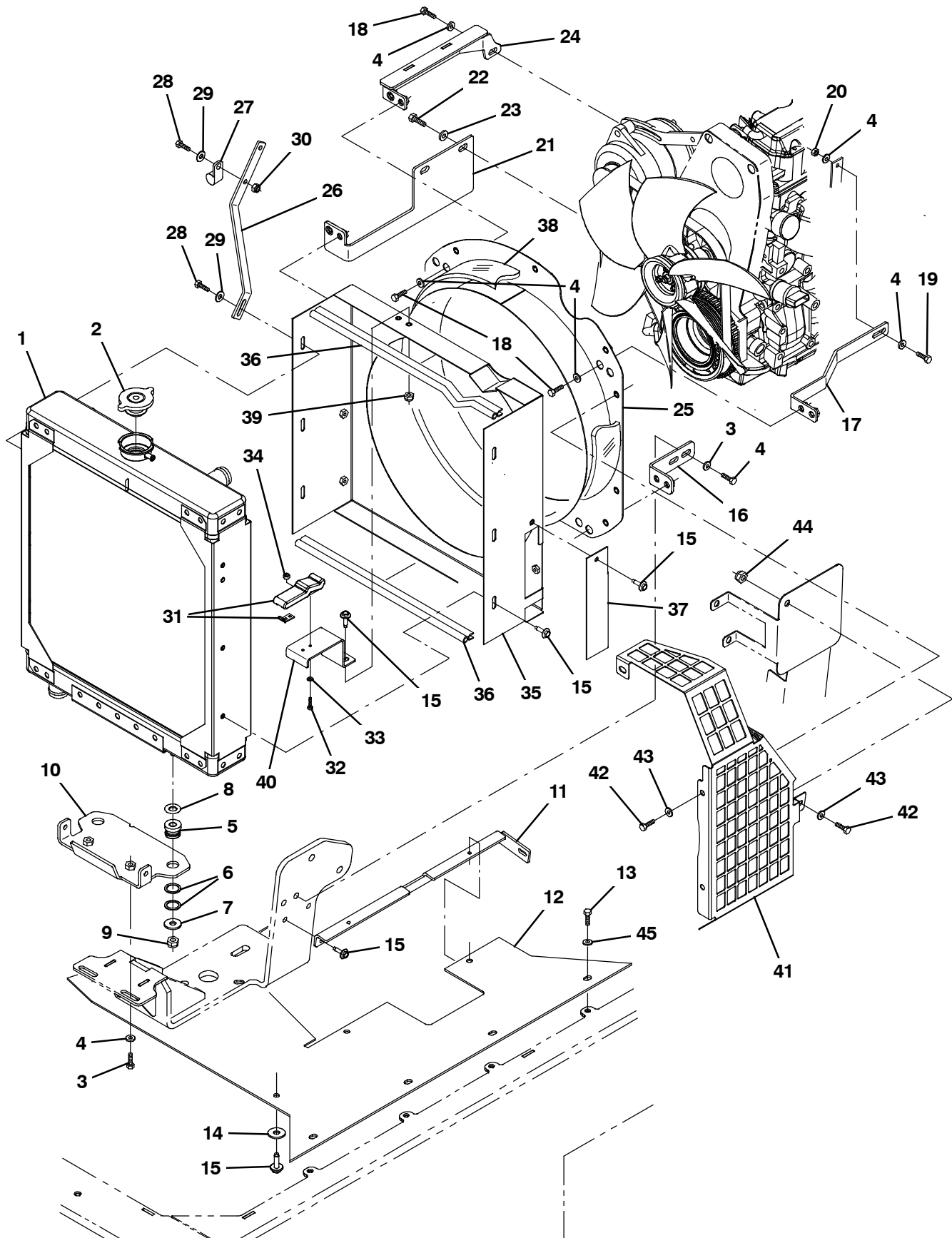
Fig. 21 - GM Engine Radiator and Mount Group (000000-001249)
