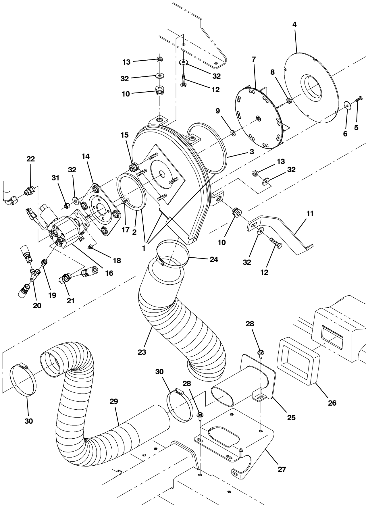
Fig. 64 - Vacuum Fan Group, Sweeping
