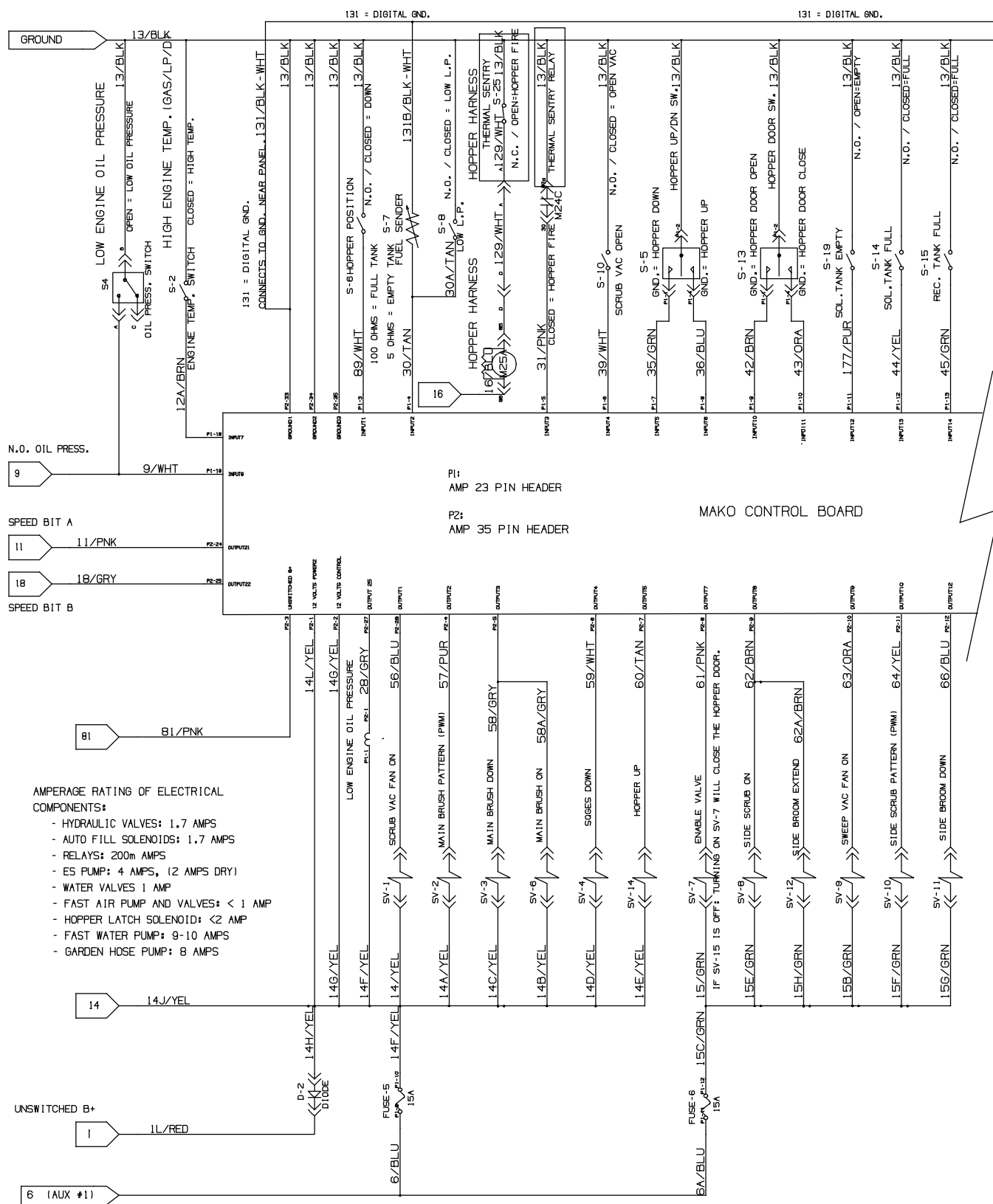
Fig. 76 - GM Electrical Schematic (001545-003999) (3 of 7)
