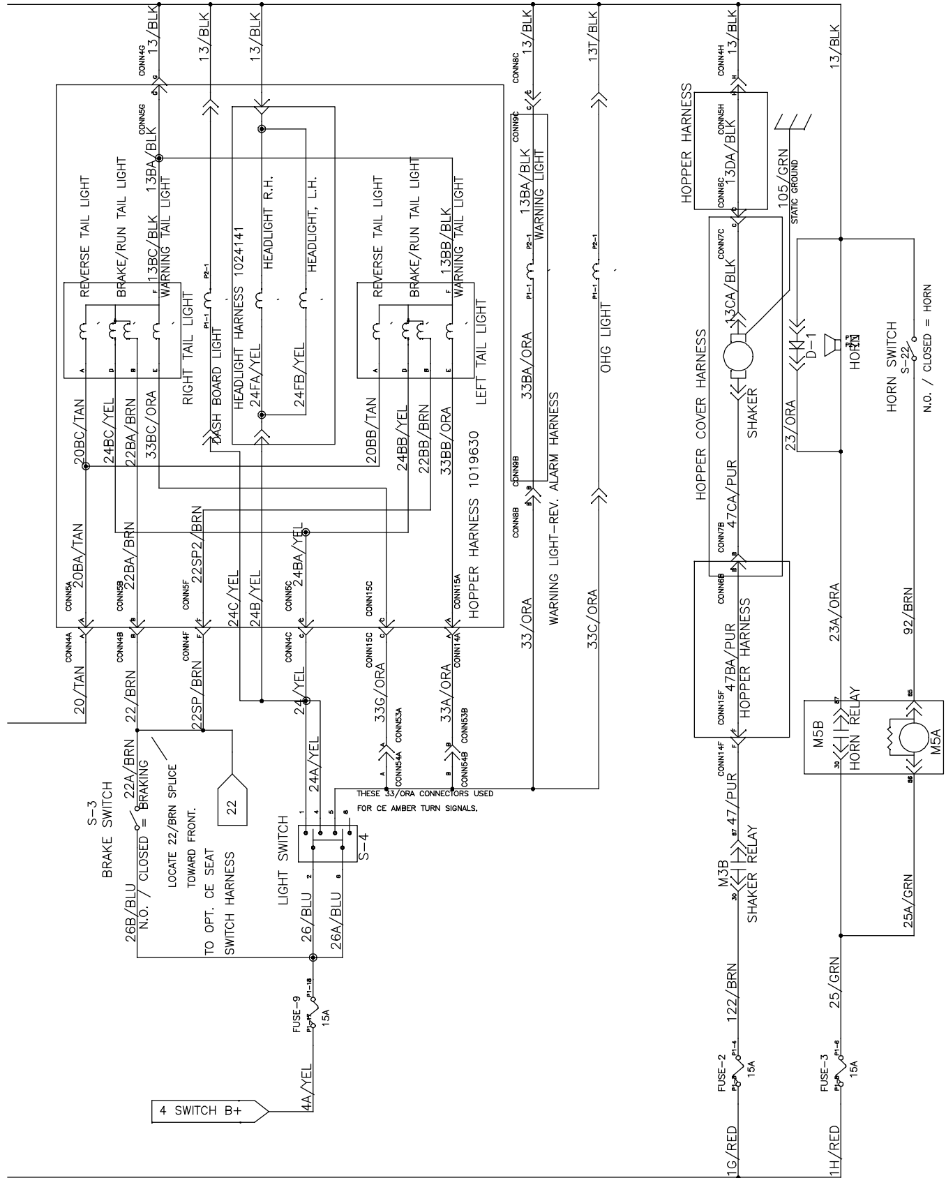
Fig. 75 - GM Electrical Schematic (000000-001544) (2 of 7)
