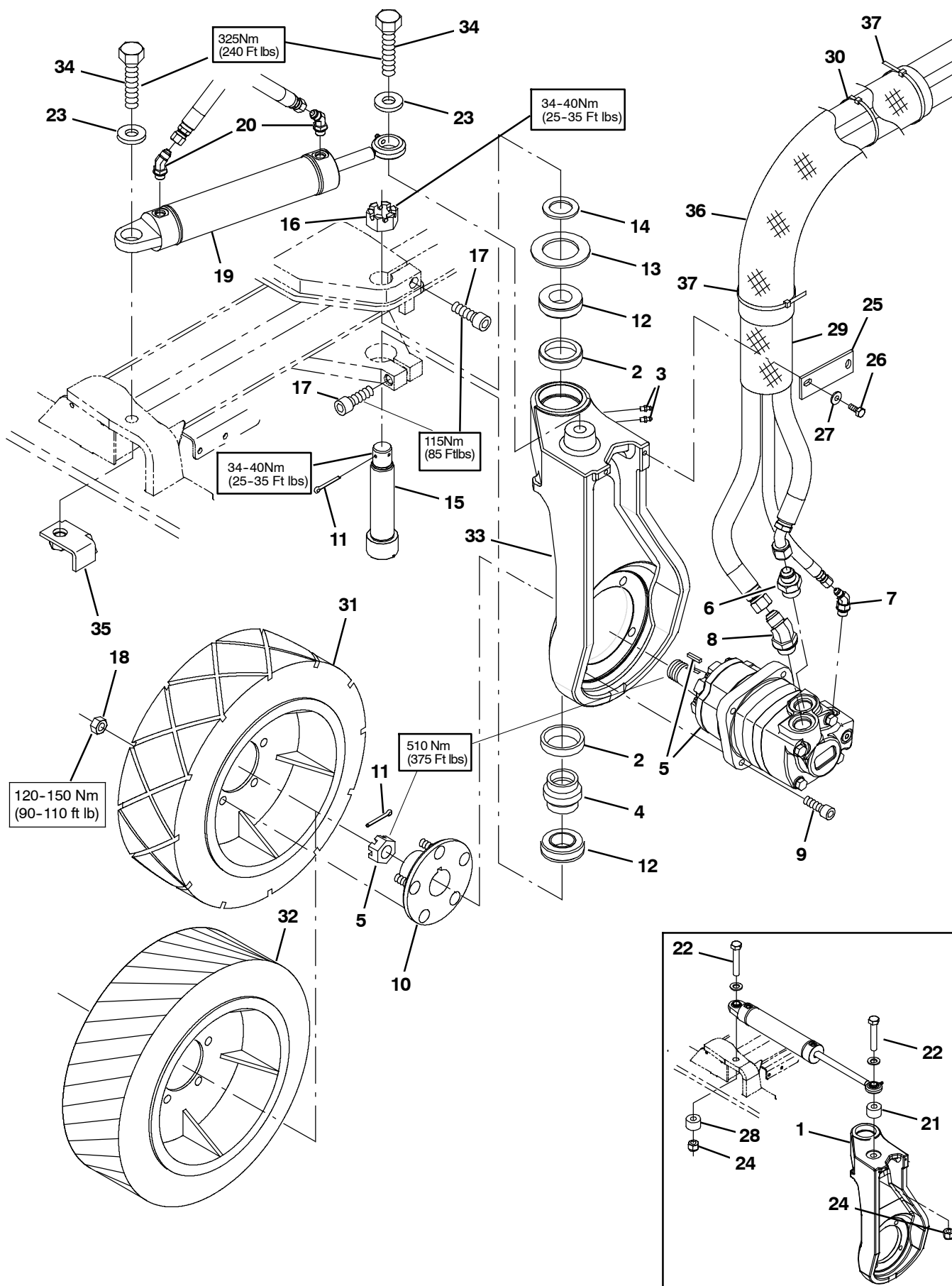
Fig. 37 - Wheel Group, Front Drive
