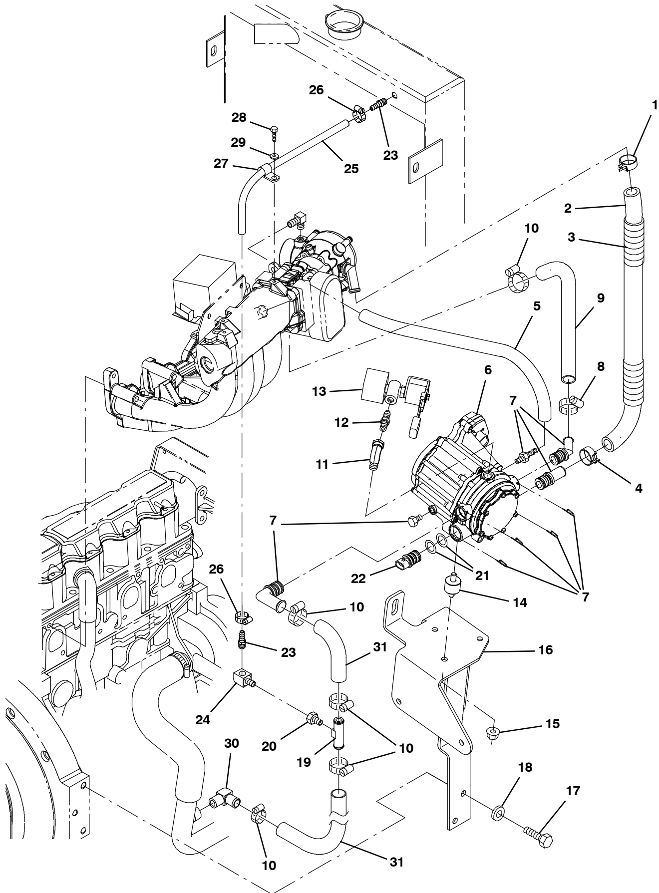
Fig. 15 - GM Engine Vaporizer Group, LPG (000000-001320)
